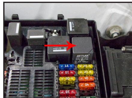
04-10 Jaguar XJ Series Relay located on the right side of the vehicle in the engine compartment.
